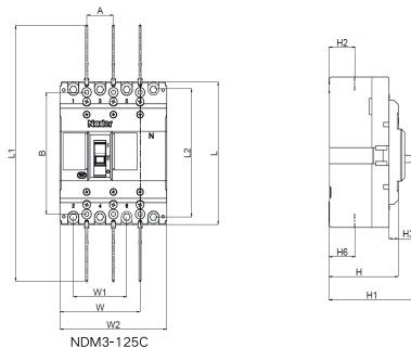
图 2 板后接线/ Fig 2 Rear-plate connection
